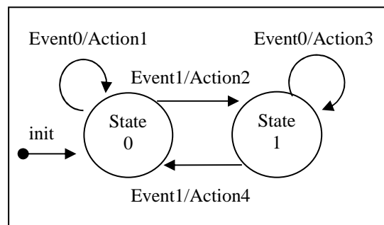
Gambar 1. Diagram state sederhana (Sumber: Setiawan, 2006)
