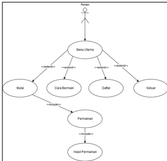
Gambar 4. Use Case Diagram Permainan “The Relationship”
